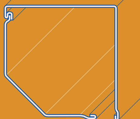
2 PARTS BOX 45°
