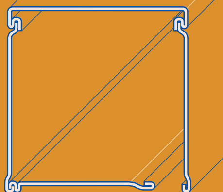
4 PARTS ALUMINIUM BOX
