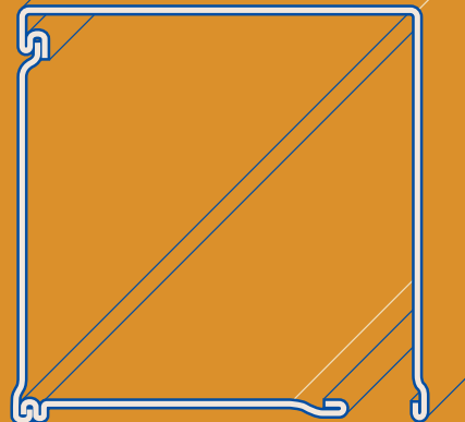
3 PARTS ALUMINIUM BOX
